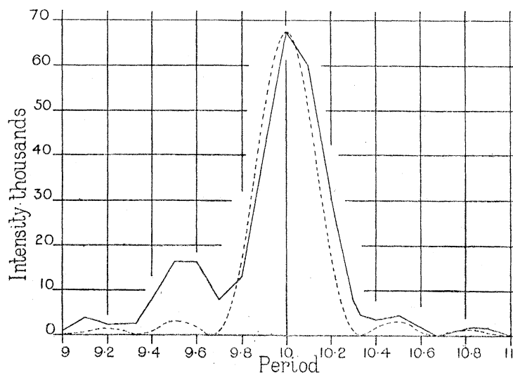
FIG. 7.—Periodogram for the experimental disturbed series on which fig. 2 is based : data in Table VI.
